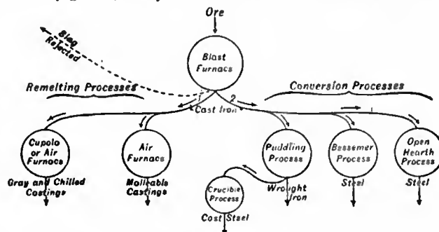
FIG. 6.—General Scheme of Iron Manufacture.
