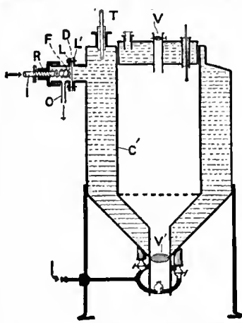
FIG. 8.—D'Arsonval Incubator.
