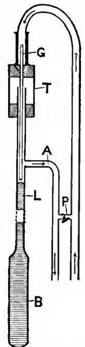
FIG. 15.—Page's Thermostat.
