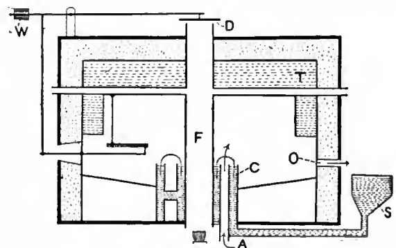
FIG. 6.—The Winchcombe Incubator.
