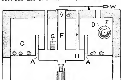
FIG. 7.—Hillier's Incubator.
