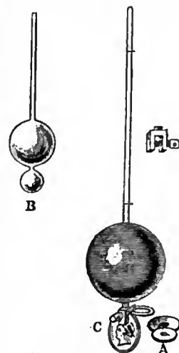
FIG. 1.—Boyle's New Essay Instrument.
