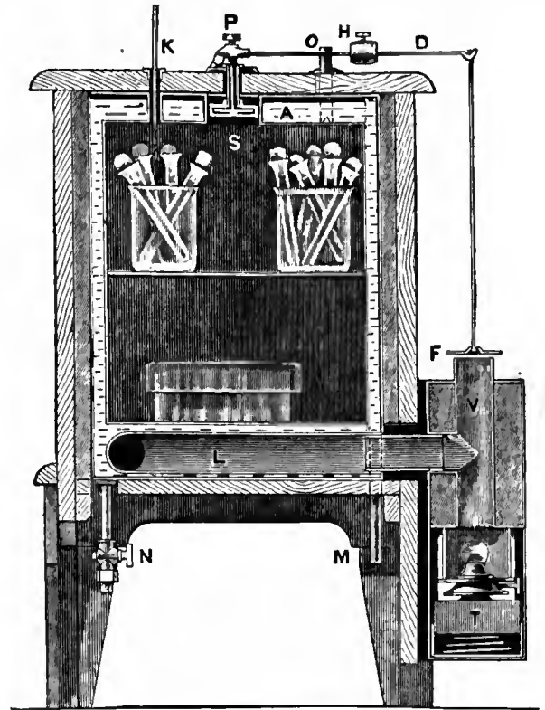
FIG. 9.—Hearson's Bacteriological Incubator. (Heated by a petroleum lamp.)
