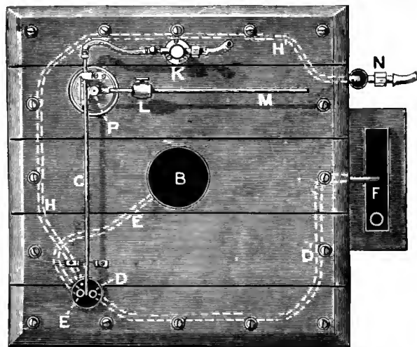
FIG. 12.—Hearson's Cool Biological Incubator.
