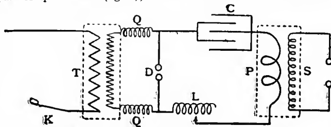
FIG. 2.—Arrangements for producing High Frequency Currents.
