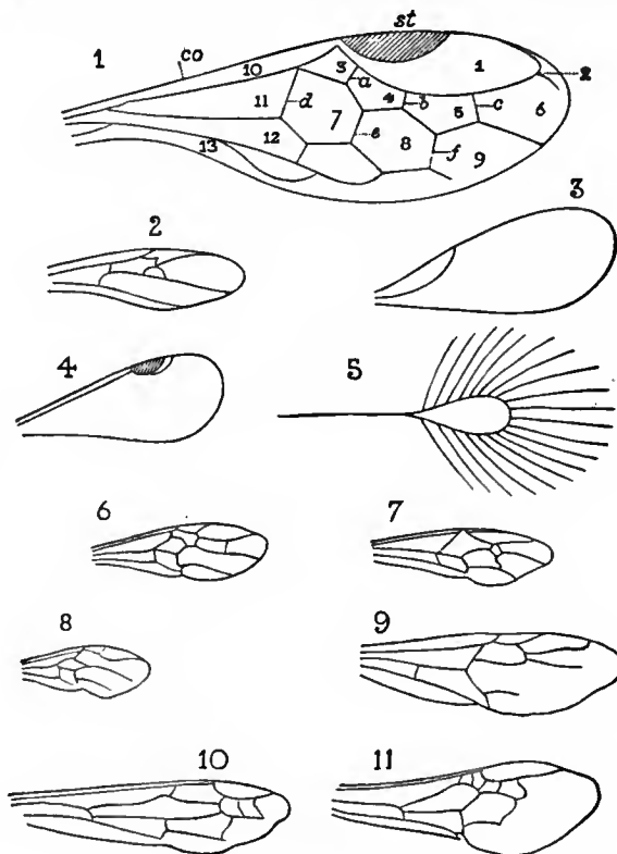
FIG. 4.—Fore-Wings of Hymenoptera.
